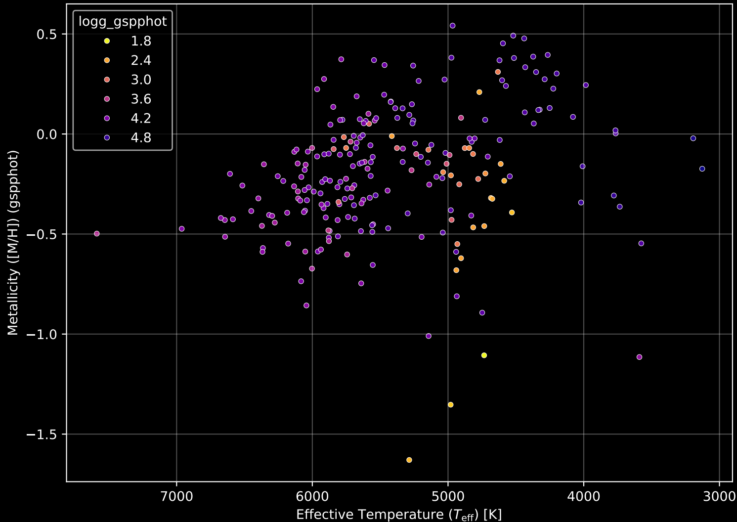
APOGEE DR17 Field: [172+63_MGA] Stellar Population Parameters (n= 230)
