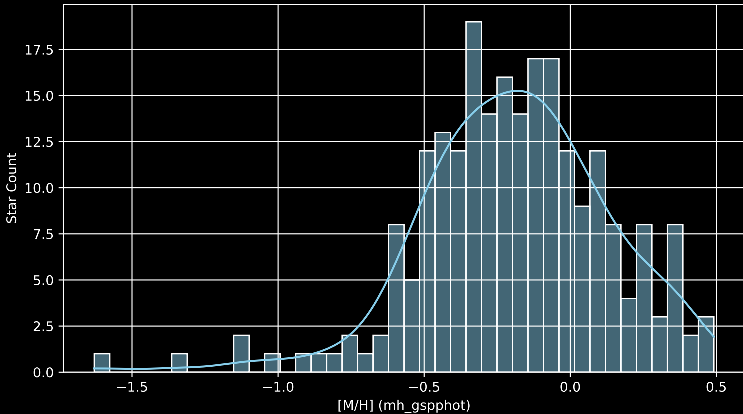
APOGEE DR17 Field: [172+63_MGA [M/H] (mh_gspphot) (n= 229)
