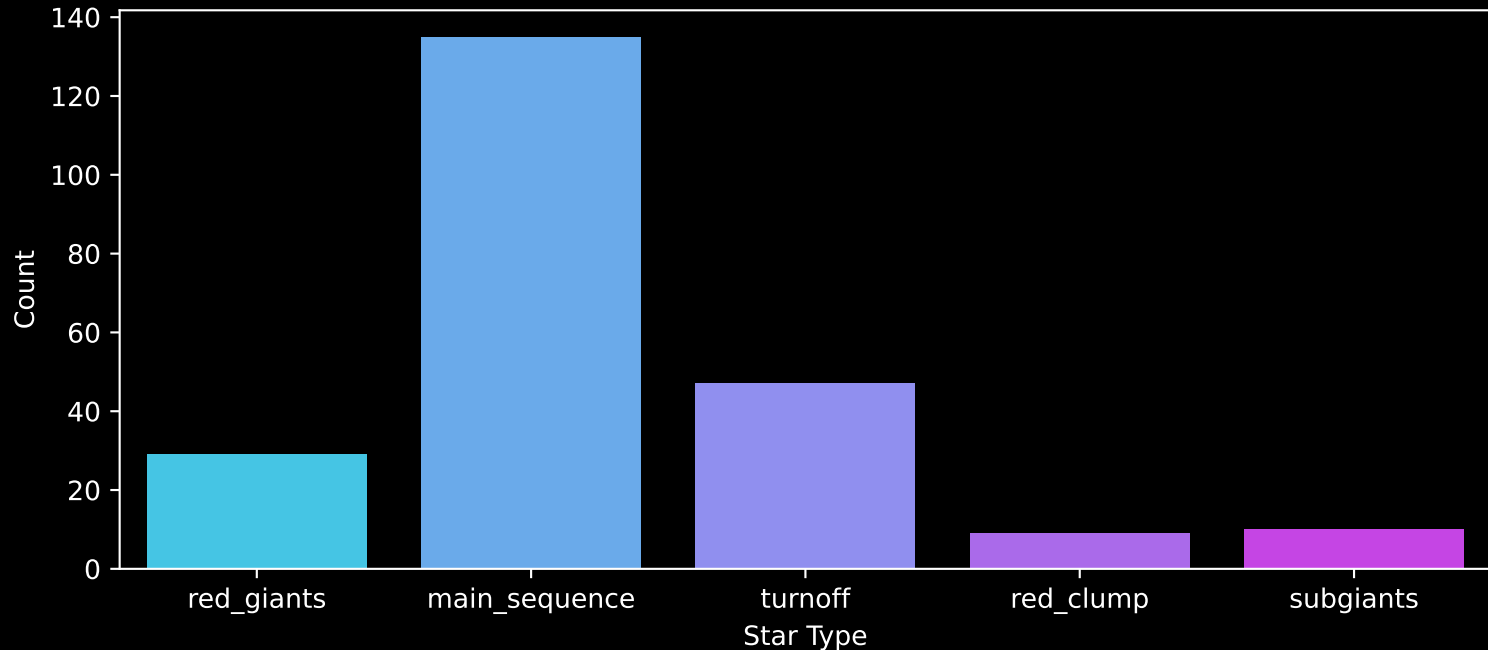
APOGEE DR17 Field: [172+63_MGA] Count plot of Star Type
