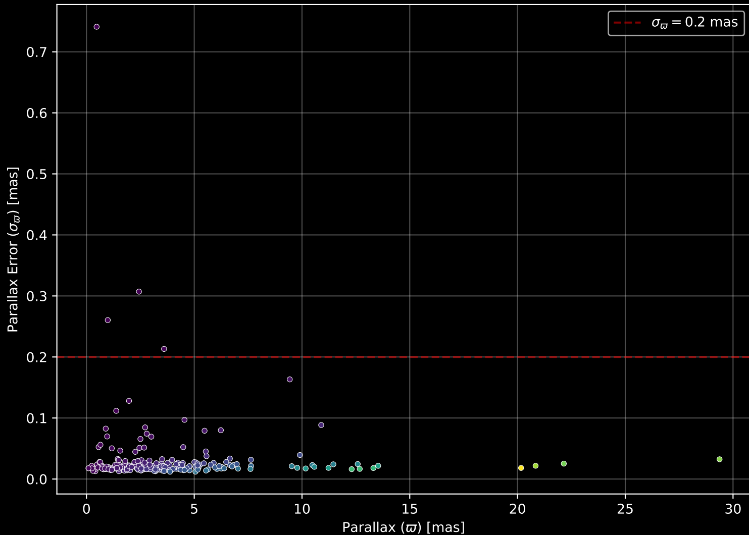
APOGEE DR17 Field: [172+63_MGA] Parallax Quality (n= 230)
