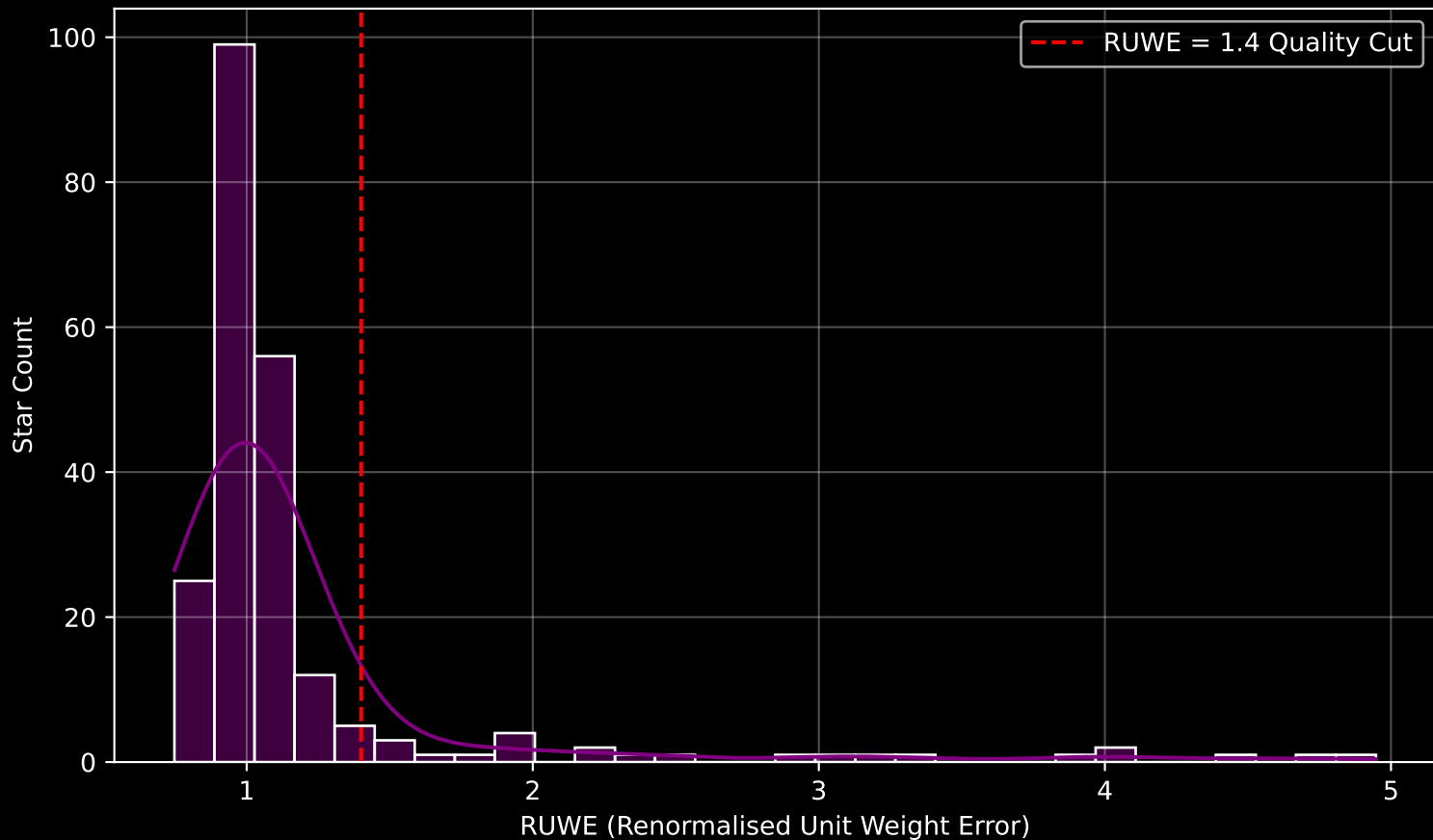
GAPOGEE DR17 Field [172+63_MGA] RUWE Distribution (n= 220)
