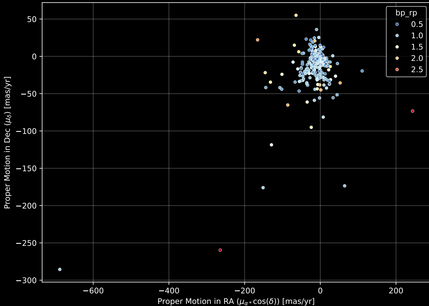
APOGEE DR17 Field: [172+63_MGA] Proper Motion Diagram (n= 230)
